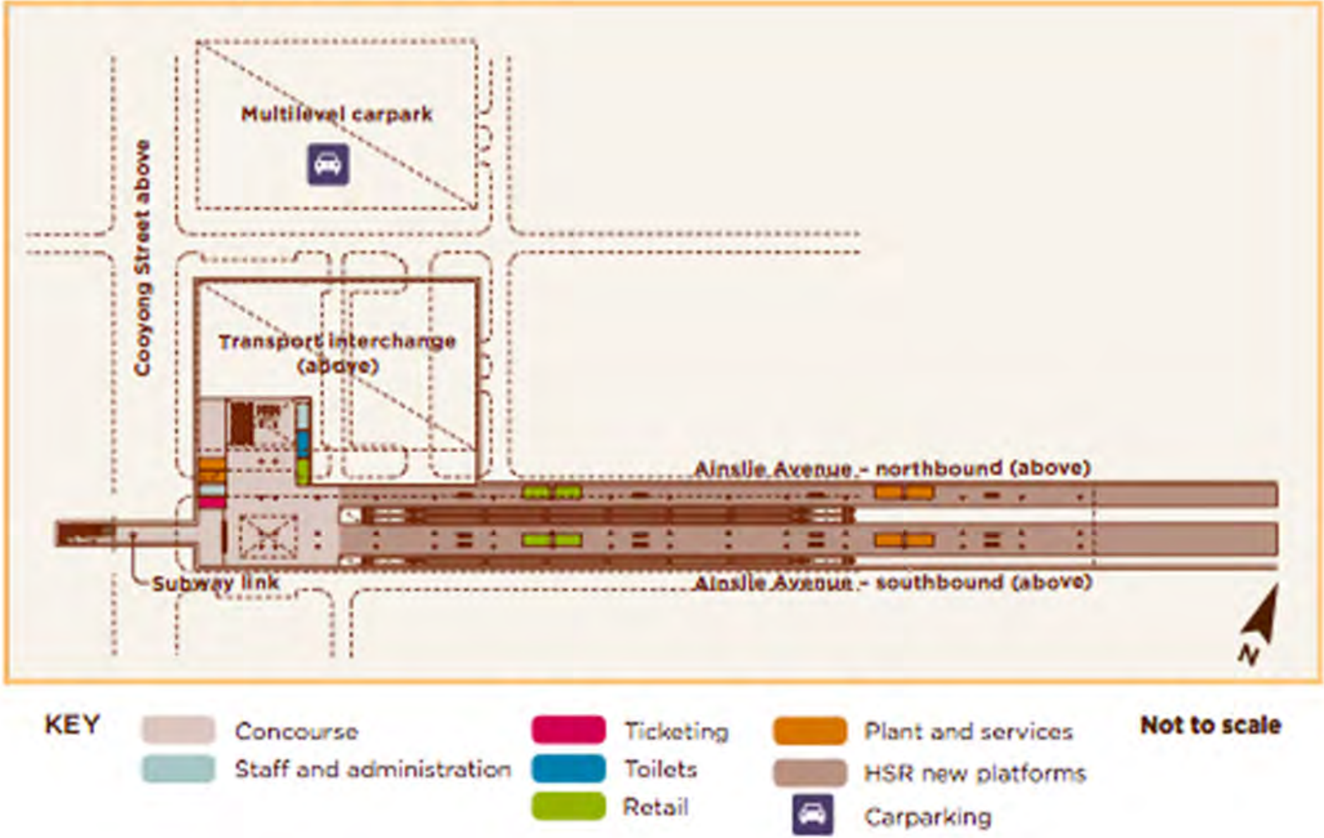
Figure 5-28 Canberra HSR station platform level plan
