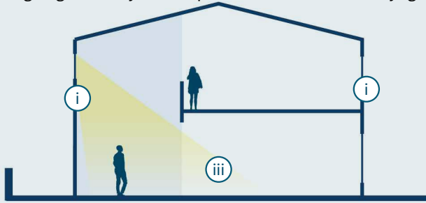
Figure 91: High placement of windows in double-height spaces can provide daylight deep into the building, and provide outlook from the upper level but privacy at the lower level.
