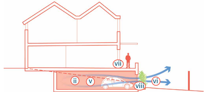
Figure 60: For basement and sub-basement car parking, using landscape screening at openings facilitates natural cross ventilation.
