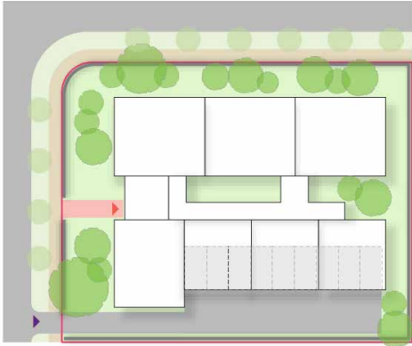
Figure 37: Apartment on large corner site with shared parking to side boundary. This maintains the prominence of the street corner.
