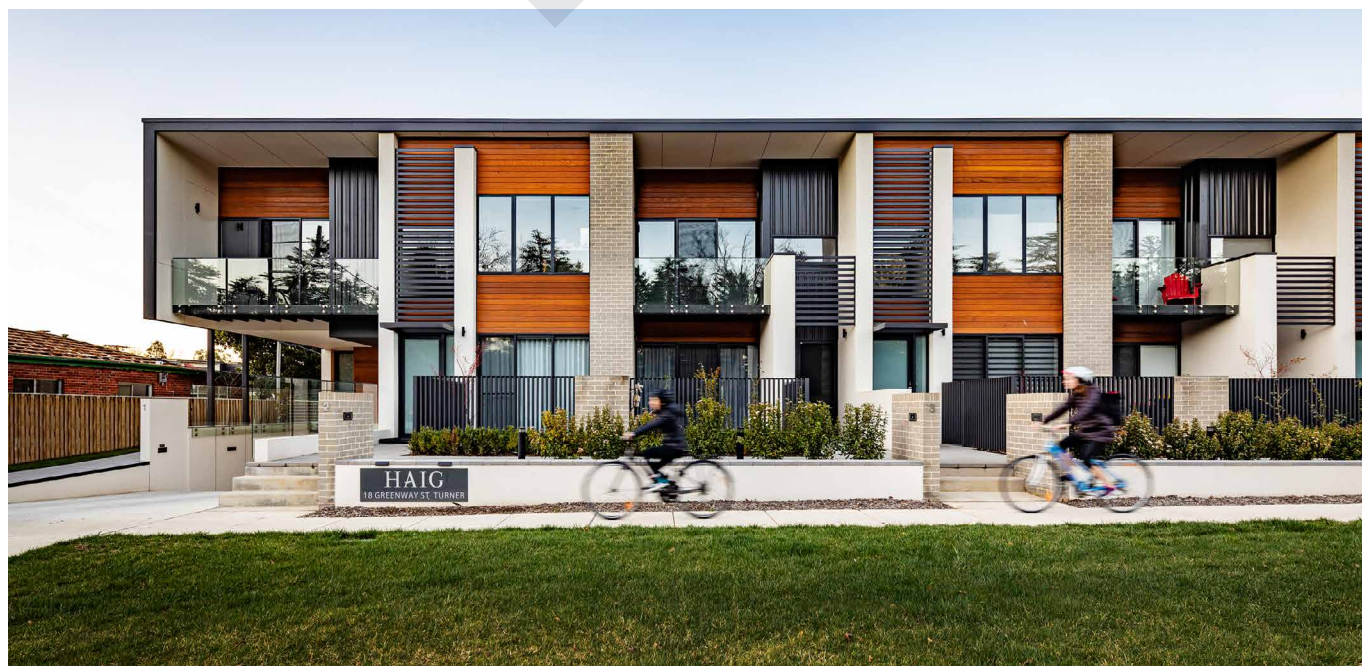
Photo 2: Apartment typology with separate pedestrian and vehicle access from the street. The ground level is slightly elevated from the street to increase the privacy of residents.
