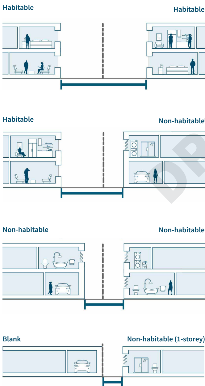
Figure 76: Indicative building separation distances between habitable and non-habitable rooms at single and multi-storeys.
