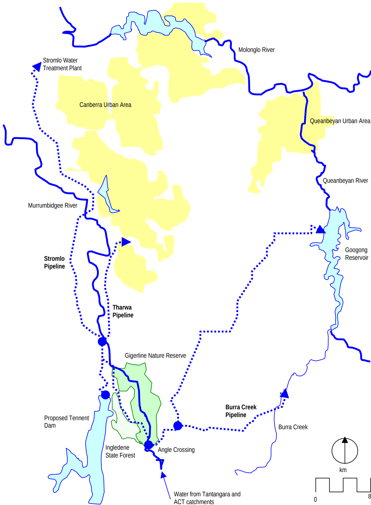
Figure 6.3: Pipeline routes
