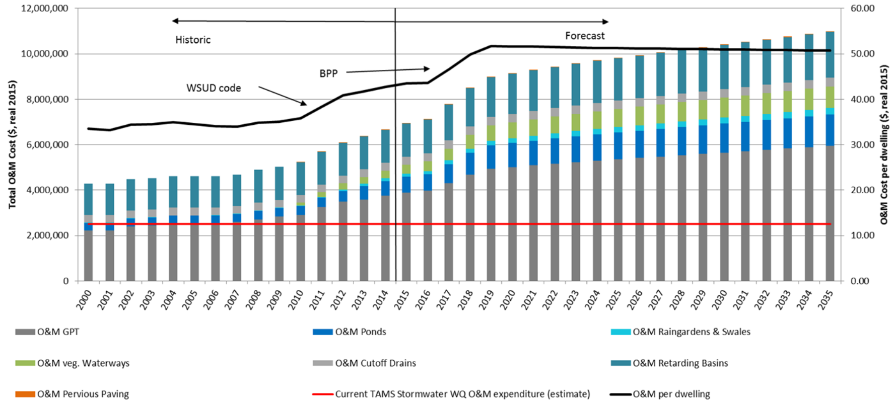
Figure 8: Stormwater WQ assets O&amp;M revenue requirement
